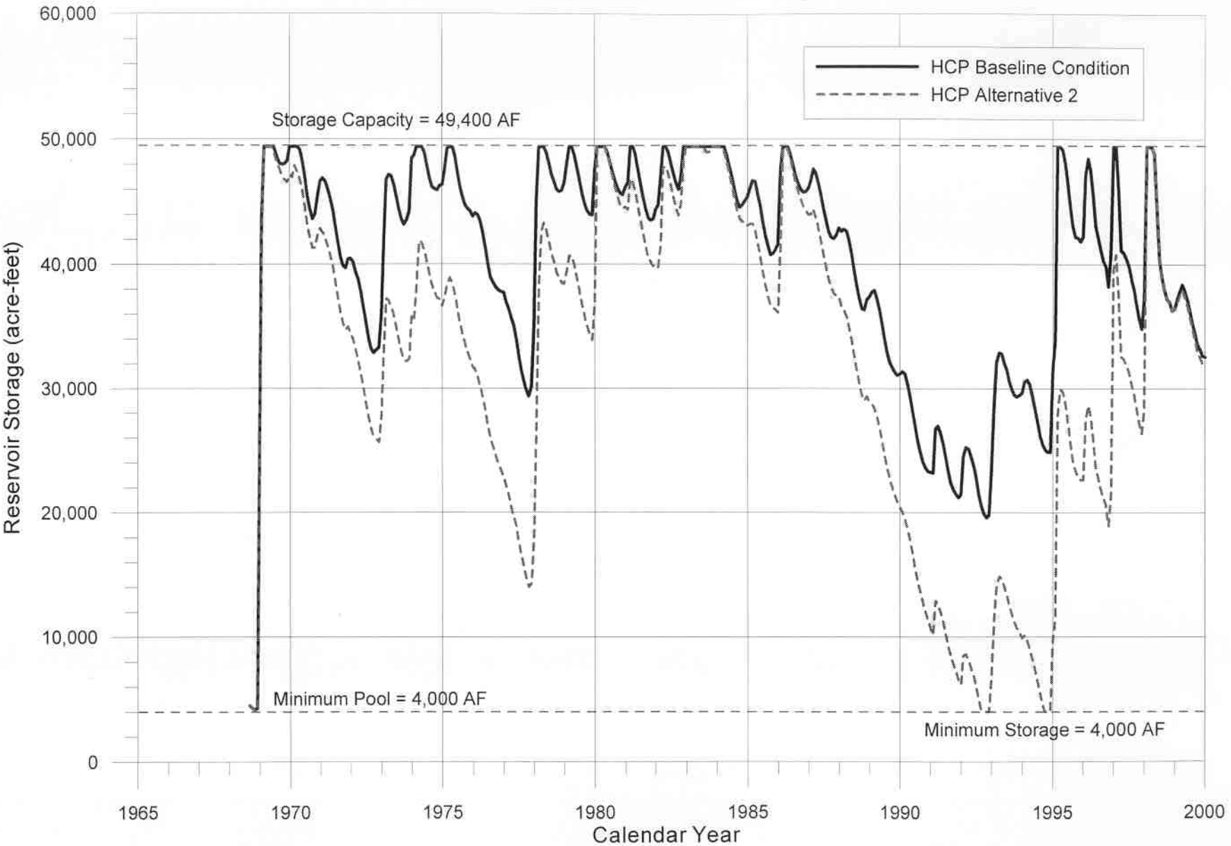
Figure 5-4 Results of Reservoir Operation Model Simulation of the Instream Flow Alternative 2 and Baseline Conditions
