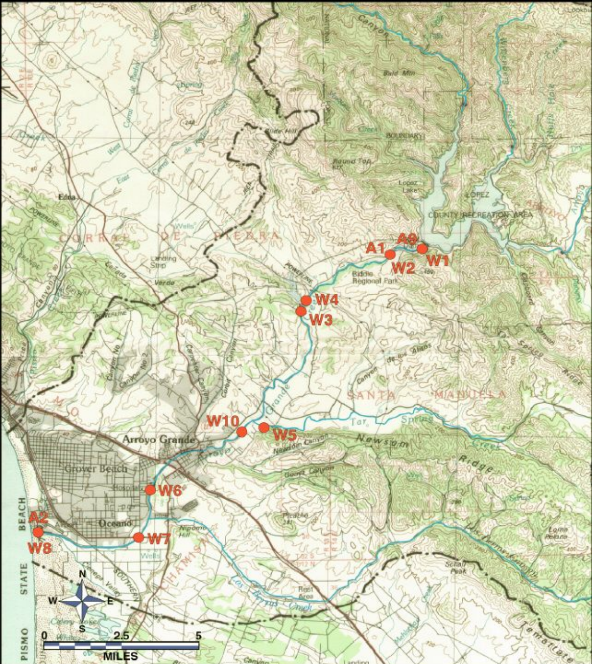
FIGURE 3-18 AIR AND WATER TEMPERATURE MONITORING LOCATIONS WITHIN ARROYO CREEK
