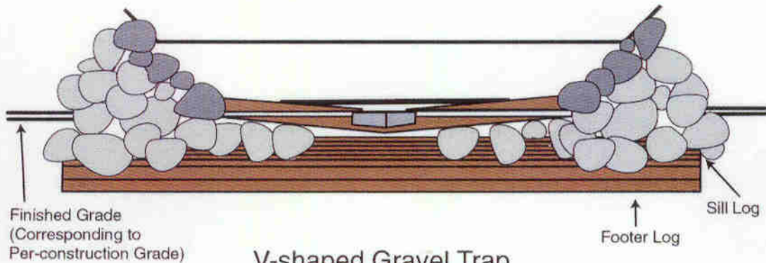
V-shaped Gravel Trap (viewed from downstream)
