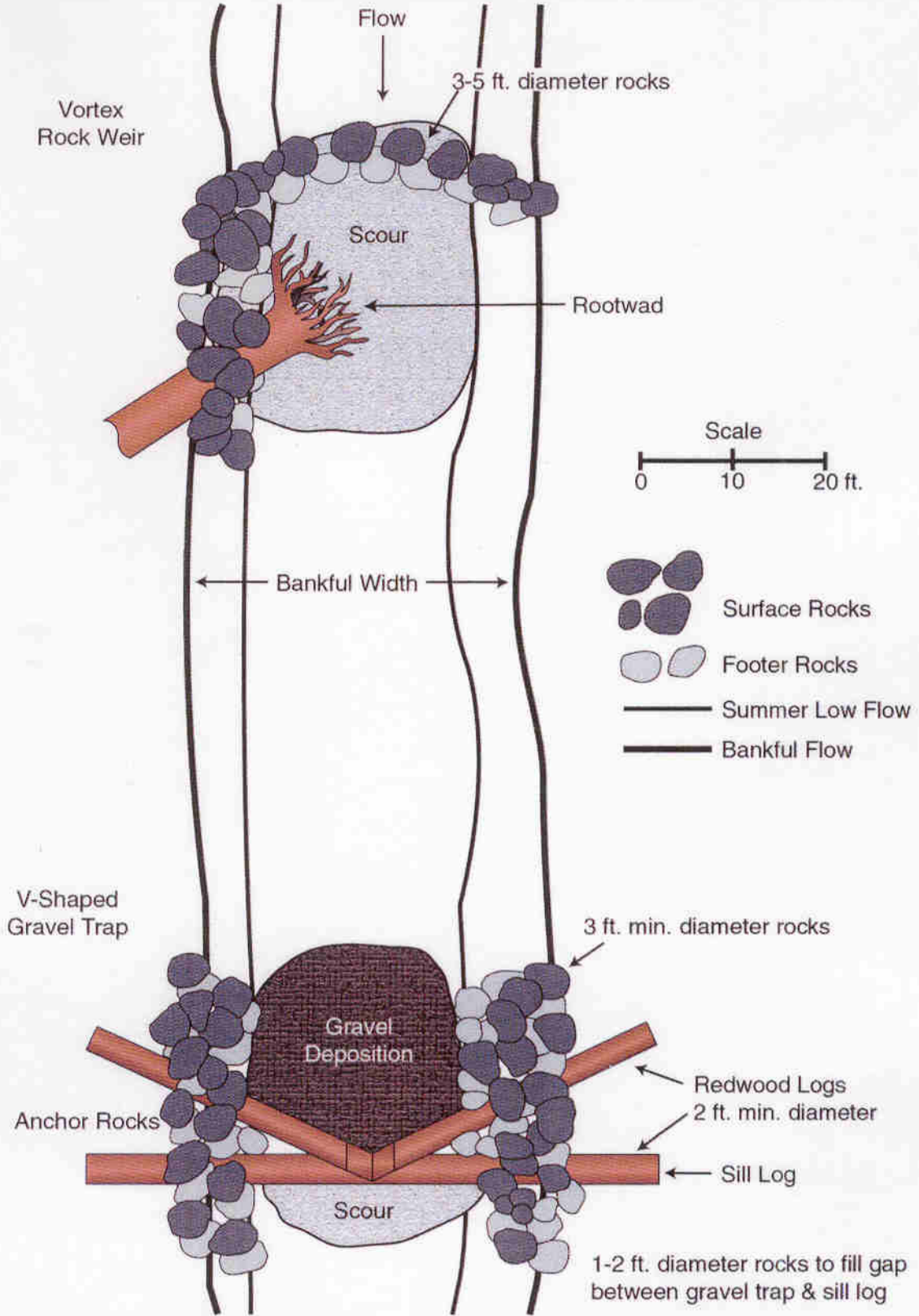
FIGURE 4-1 PLAN VIEW OF STEELHEAD HABITAT ENHANCEMENT (NON-FLOW) ACTIONS DESIGNED TO IMPROVE SUMMER POOL HABITAT AND WINTER SPAWNING GLIDES WITHIN ARROYO GRANDE CREEK. (SOURCE: ALLEY 1997).
