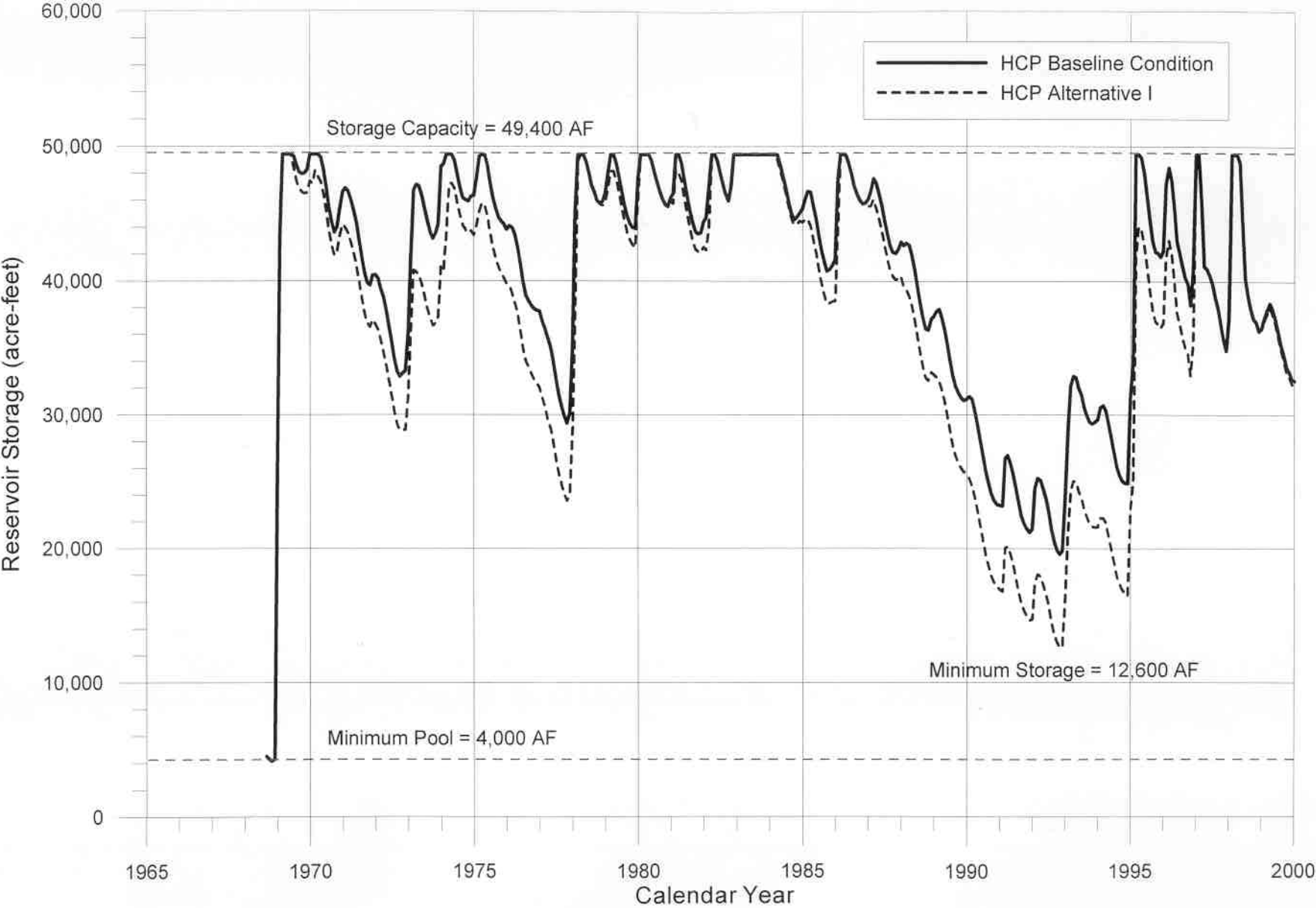
Figure 5-1 Results of Reservoir Operation Model Simulation for Proposed Alternative 1 and Baseline Condition
