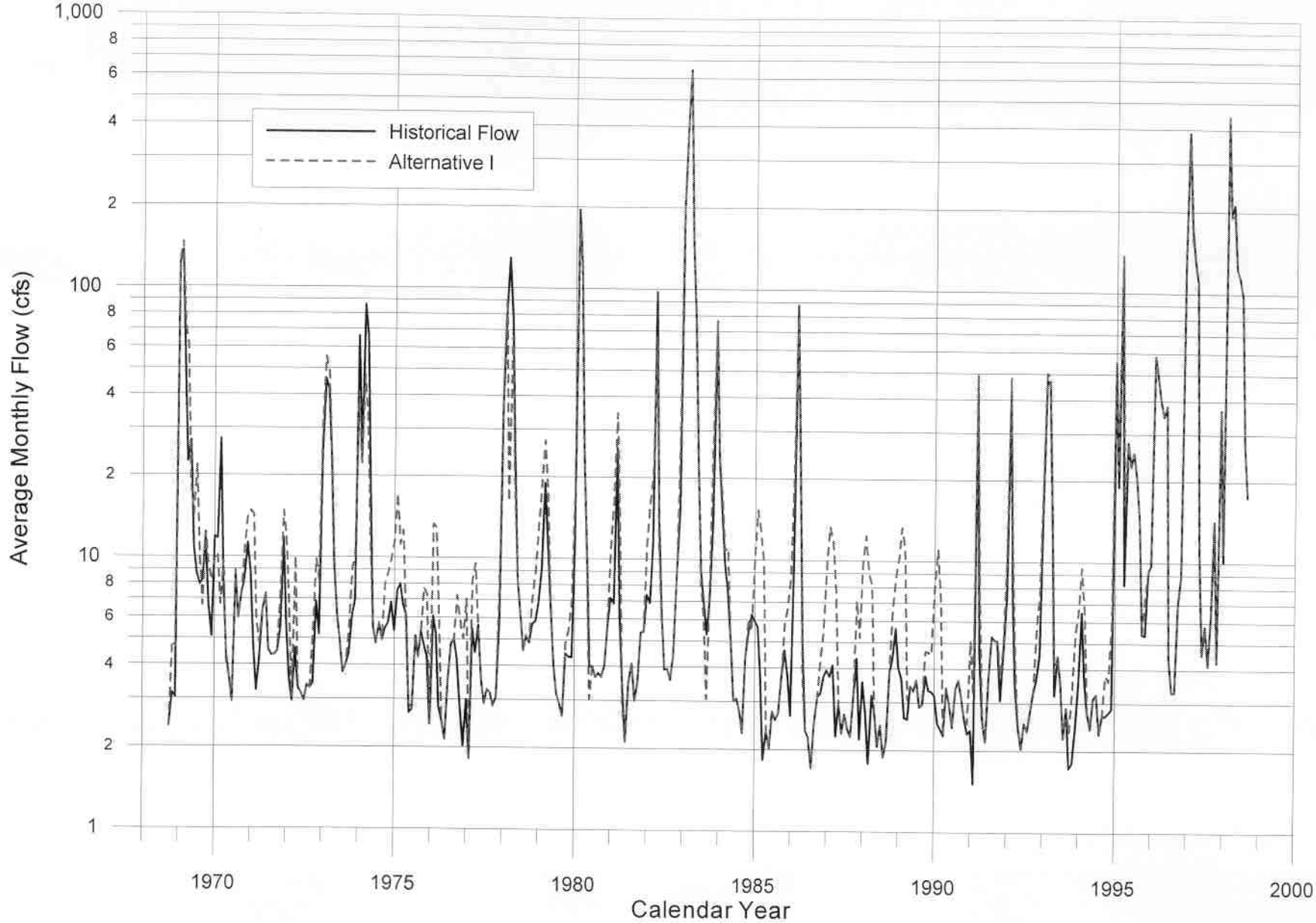
Figure 5-2 Comparison of Average Monthly Flows at Arroyo Grande Gage under the Proposed Alternative 1 and Historical Flows
